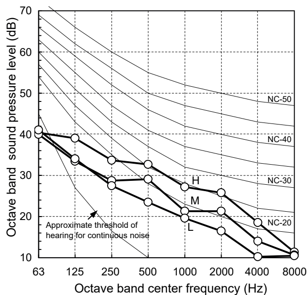
External static pressure 40 Pa
