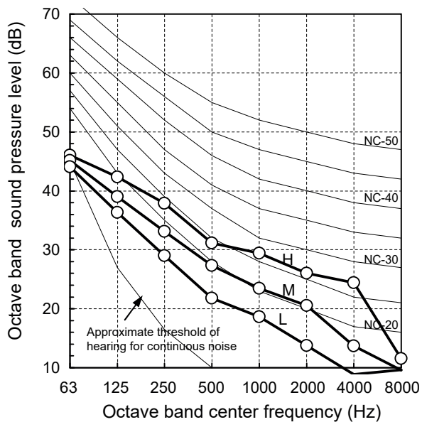
External static pressure 100 Pa
