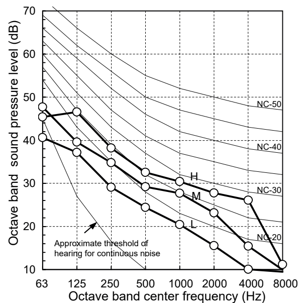
External static pressure 120 Pa
